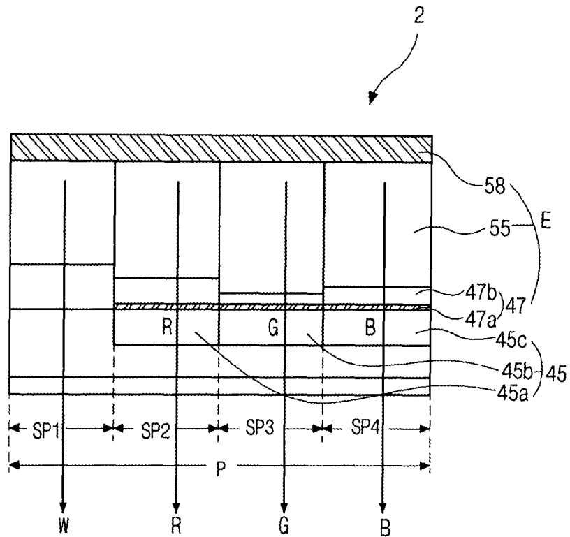
FIG. 2 Related Art
