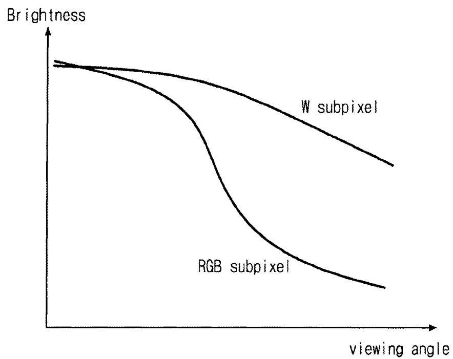
FIG. 3 Related Art
